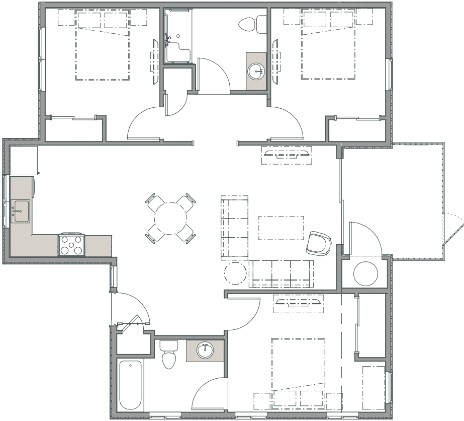
3 Bed | 2 Bath | 1158 sq.ft. EXAMPLE FLOORPLAN
